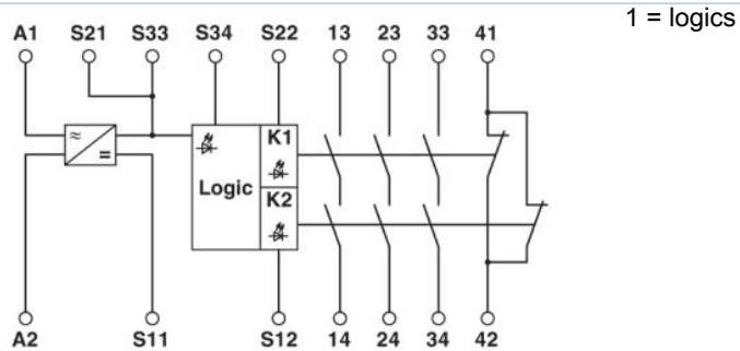
Circuit diagram
